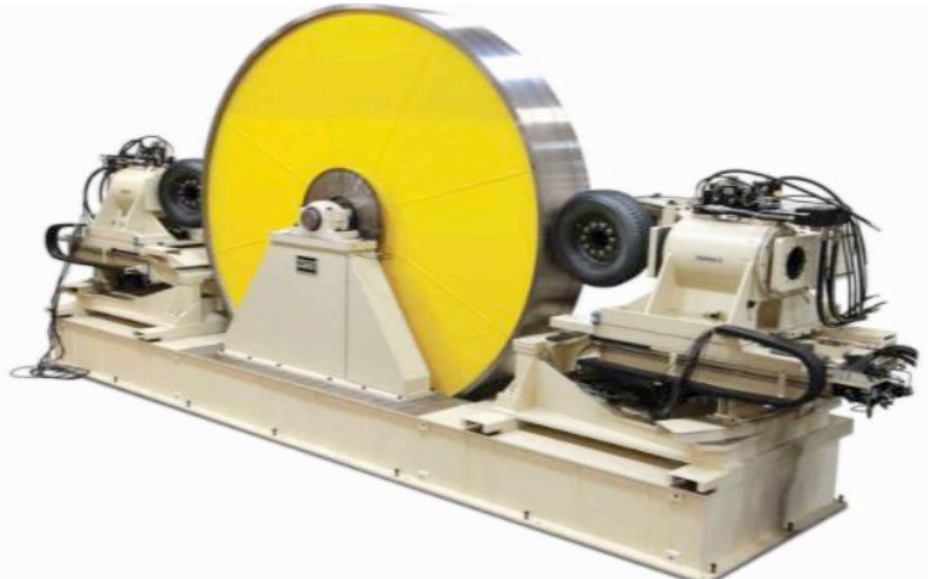
Laboratory drum method
